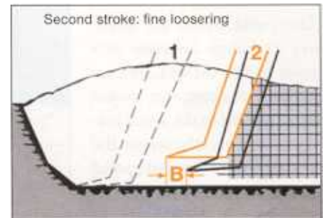
... Horizontal spades loosen the soil from above down to deep subsoils with two stroke, the first for coarse loosening the second for fine loosening
