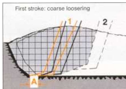
... Horizontal spades loosen the soil from above down to deep subsoils with two stroke, the first for coarse loosening the second for fine loosening
