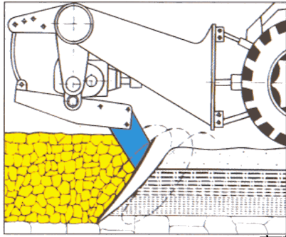
Demolition loosener in operation cutting into the ground, breaking it up and letting it fall down again with or without mixing effects
